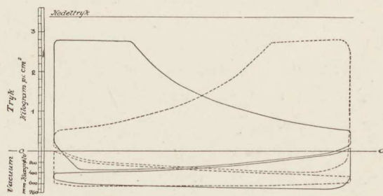
Indikatorgram, Vesterfarimagsgade.
