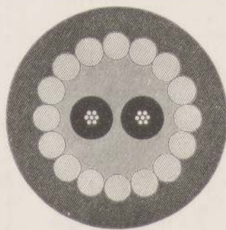
2-core Amoy Kabel (7 Tons).
