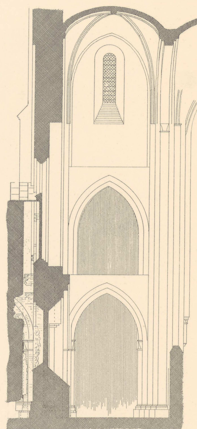
SNIT C—D.
