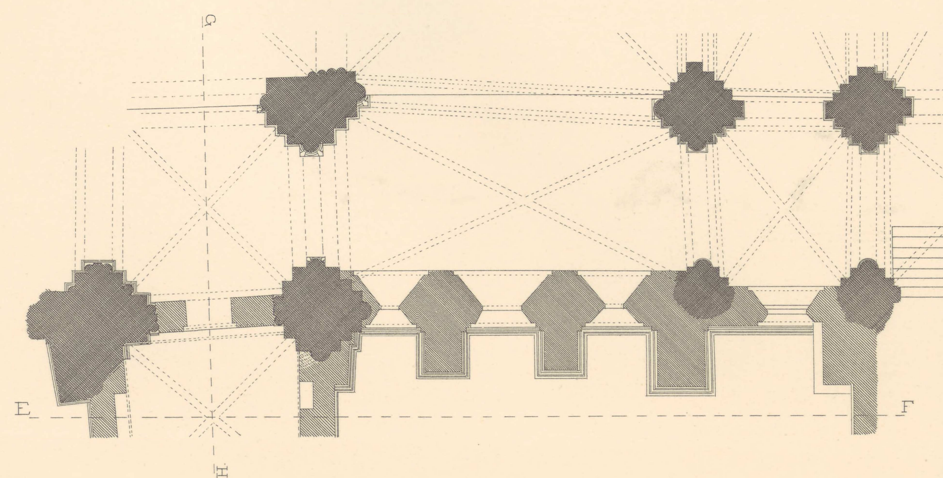
UNDERSTE PLAN.
