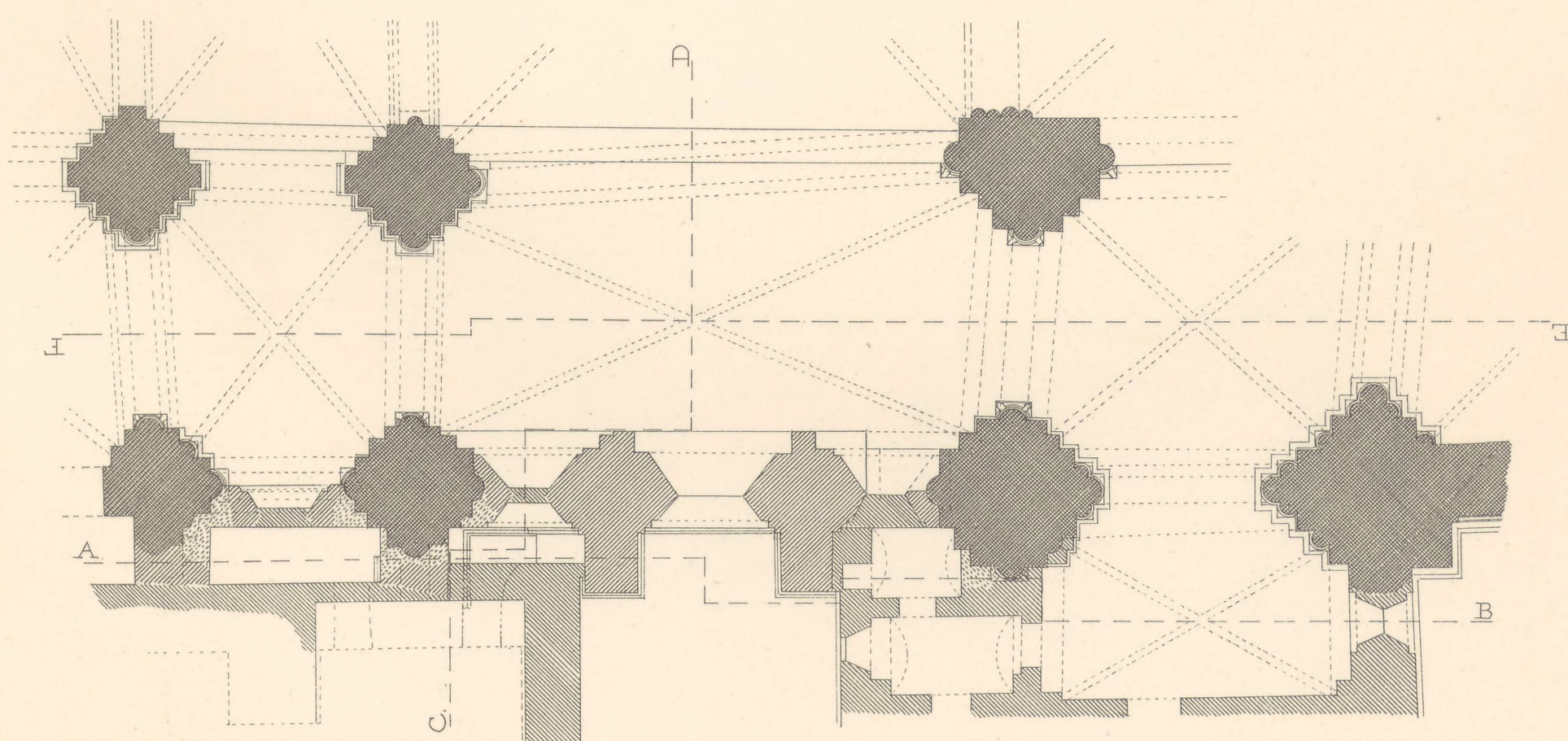
UNDERSTE PLAN.
