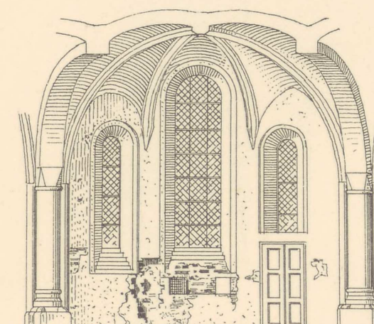
SNIT C—D.
