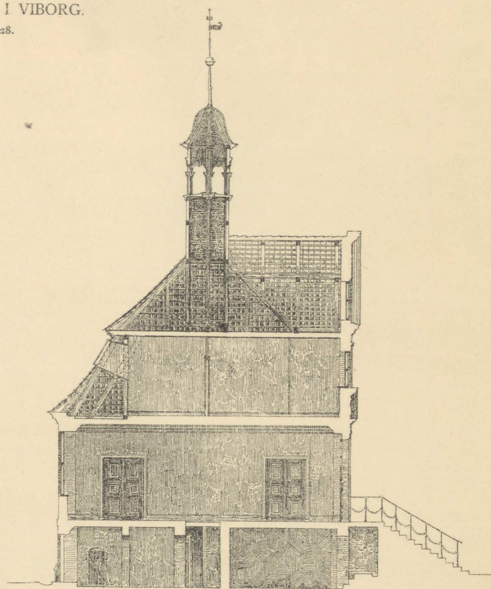
SNIT S—N
