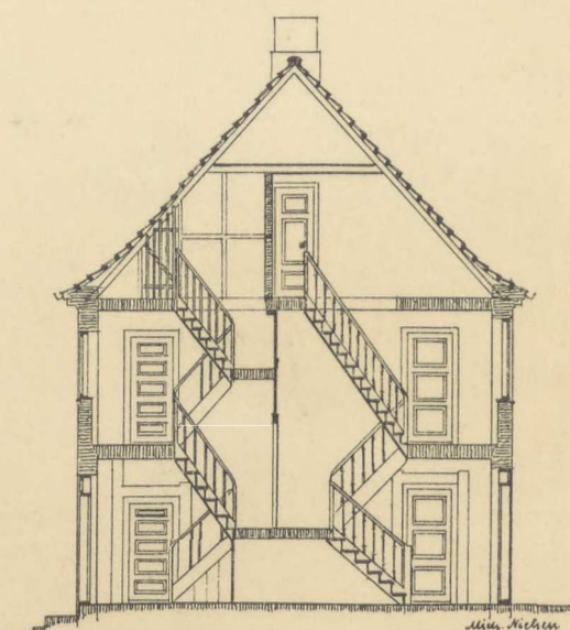
SNIT A—B.
