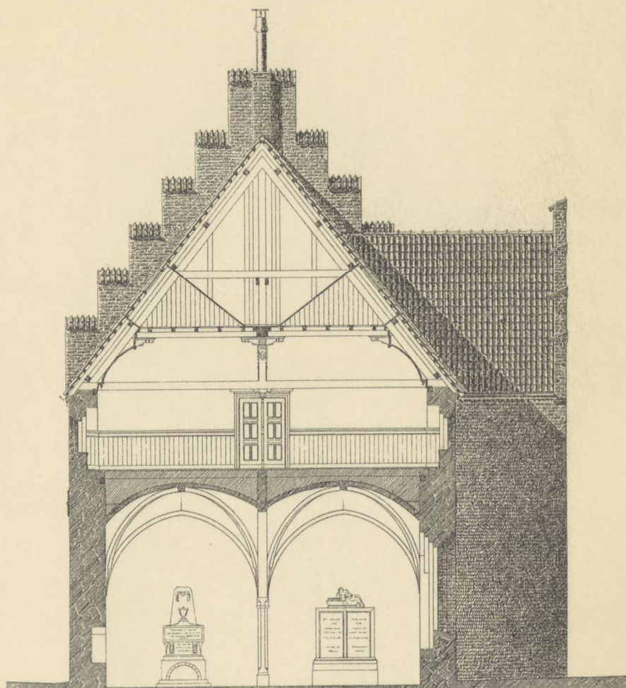
SNIT A—B
