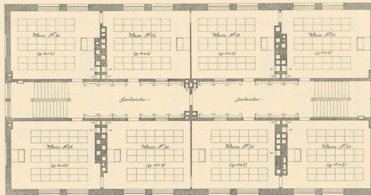
Plan of 1 st (2 nd & 3 rd ) Sal.
