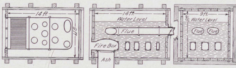
Wooden Boilers used in the Philadelphia Water Supply
