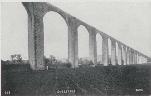
Near View of Zempoala Aqueduct, Mexico
