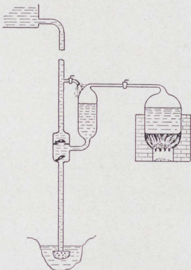
Savery's Engine
