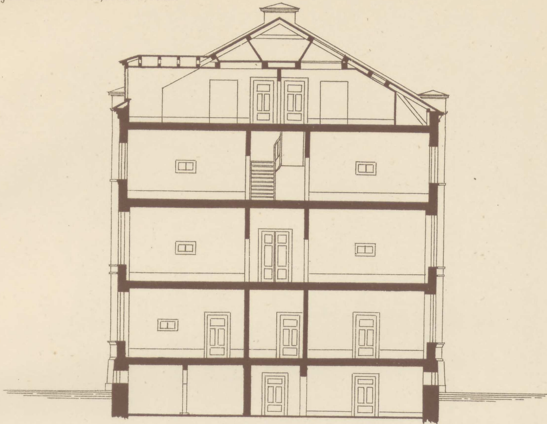
Snit
