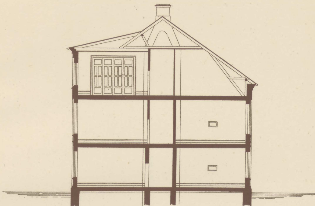
Snit
