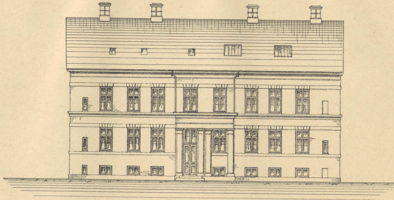
Façade mod Vest.
