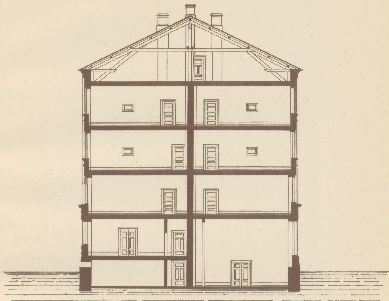
Snit
