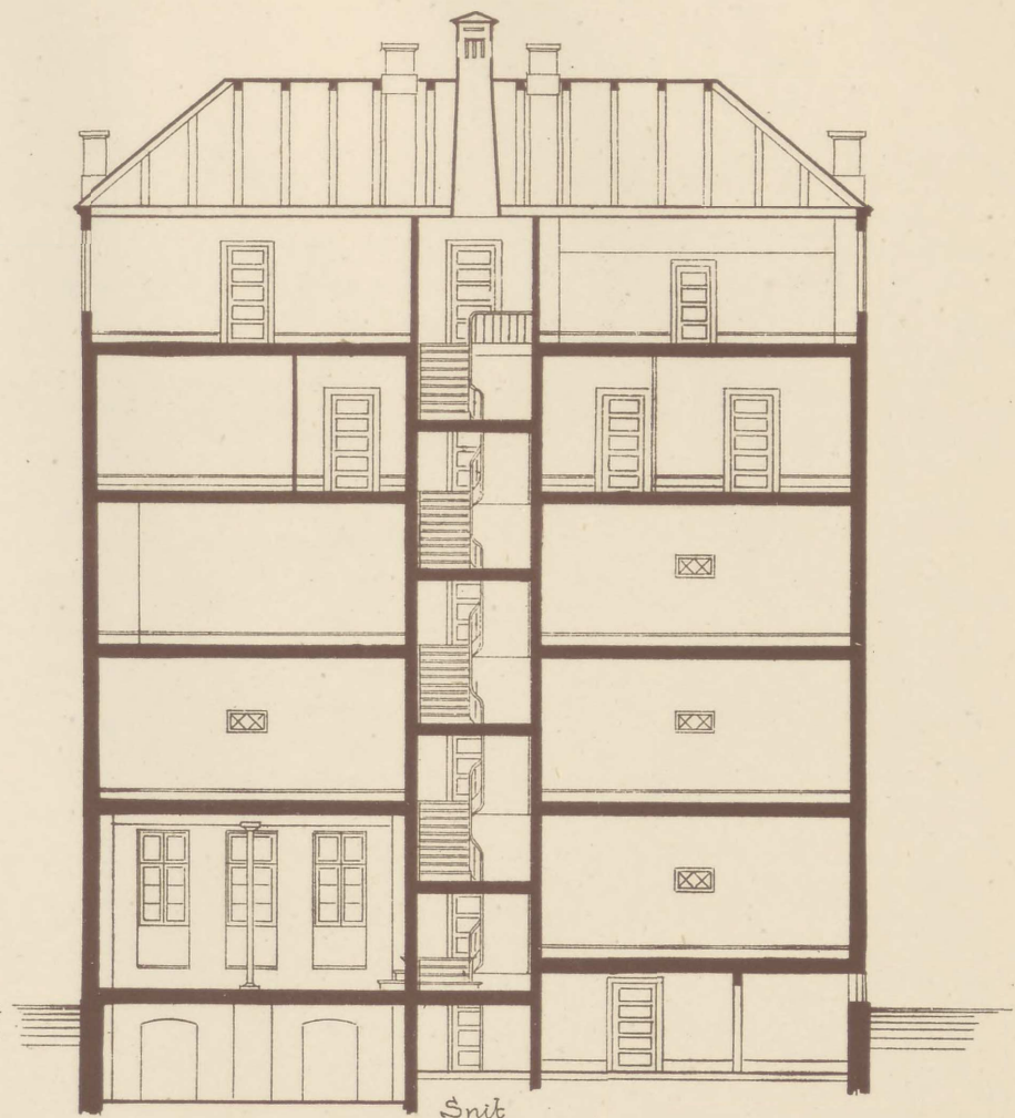
Snit
