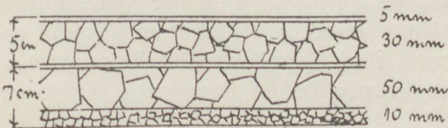
Fig. 36. Hooley's Metode.
