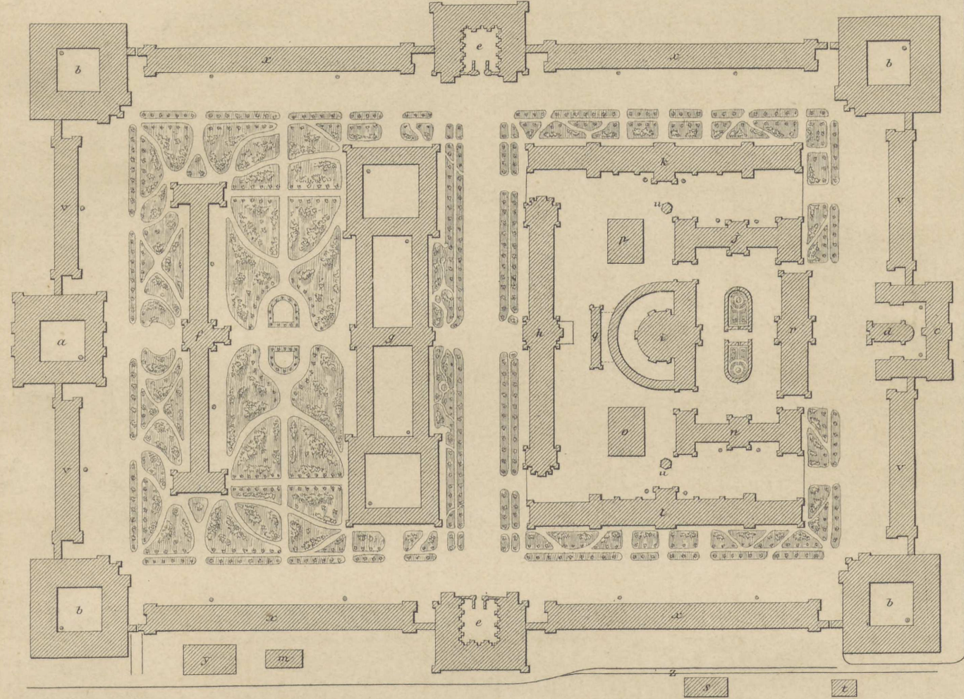
Situationsplan 1:1000
