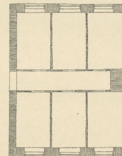
2. SALS PLAN
