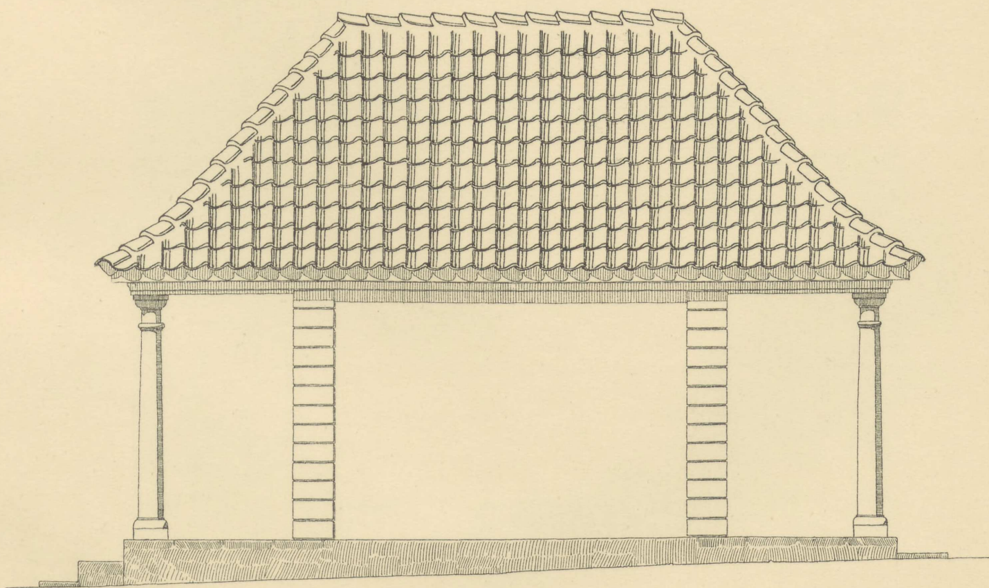
LANGSIDE.
