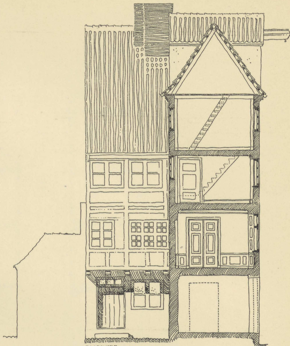
GAARDSIDE
