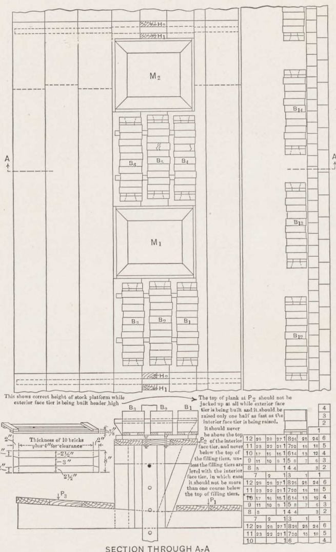
Fig. 43.—Location of the pack on the wall while building the exterior face tiers. Pack-on-the-wall method.
