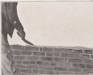
Fig. 37.—Working right to left.—Spreading mortar on the interior face tier.
