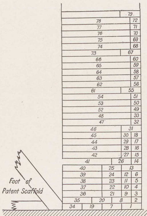
Fig. 16. — The numbers show the correct sequence of courses and tiers as laid from the non-stooping scaffold for the fewest, shortest, and most economical motions. This scaffold permits a much larger percentage of the brick to be laid as "filling in," instead of as "backing up," consequently requiring less skillful motions.
