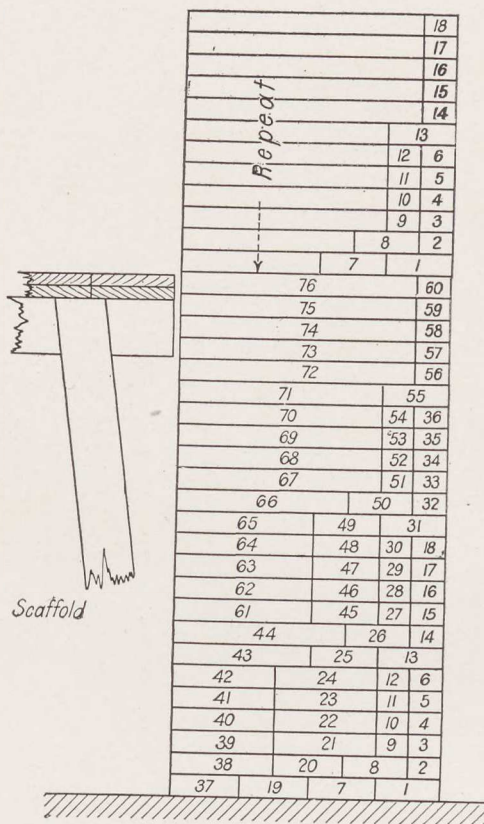
Fig. 15.—The numbers show the correct sequence of courses and tiers as laid from the ordinary scaffold for the fewest, shortest, and most economical motions.
