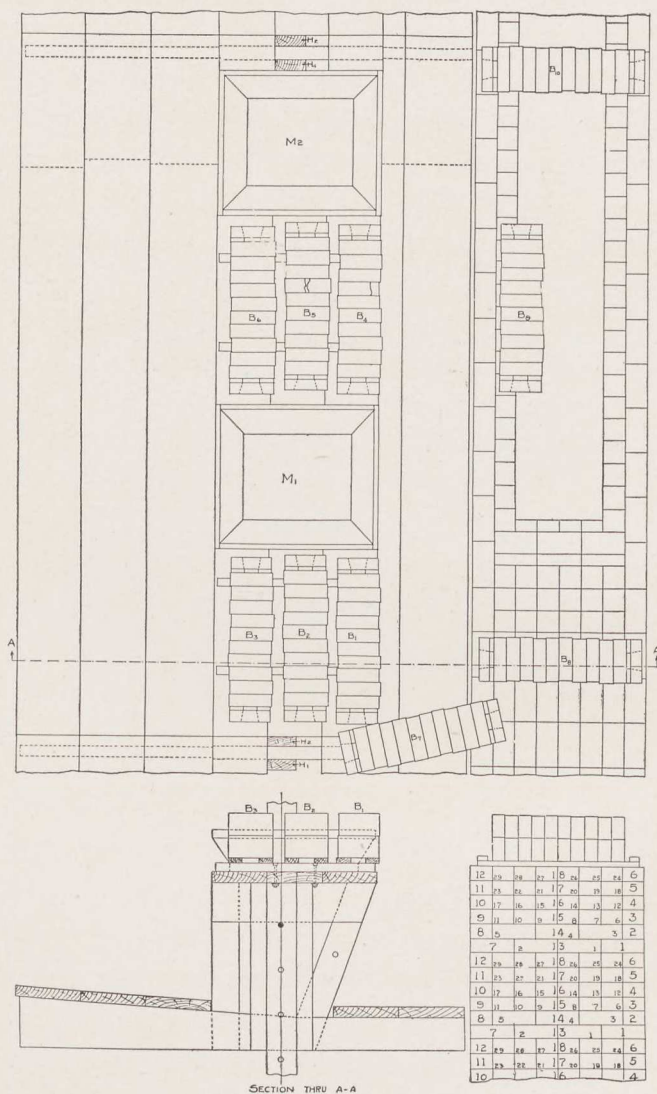
Fig. 2. — Gilbreth's patent non-stooping scaffold for bricklaying.
