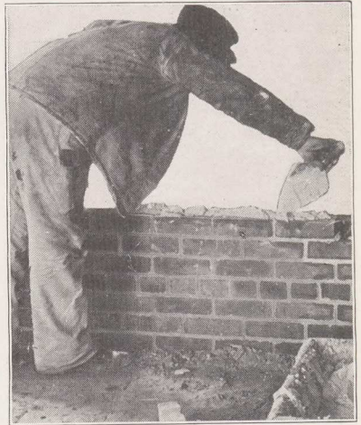
Fig. 41.—Working left to right.—Throwing mortar on the interior face tier.
