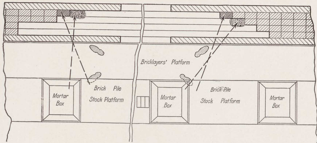
Fig. 13. — Pick-and-dip method of bricklaying on the interior or filling tiers.
