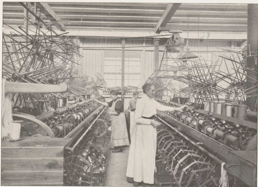
BOBBIN MASKINE
