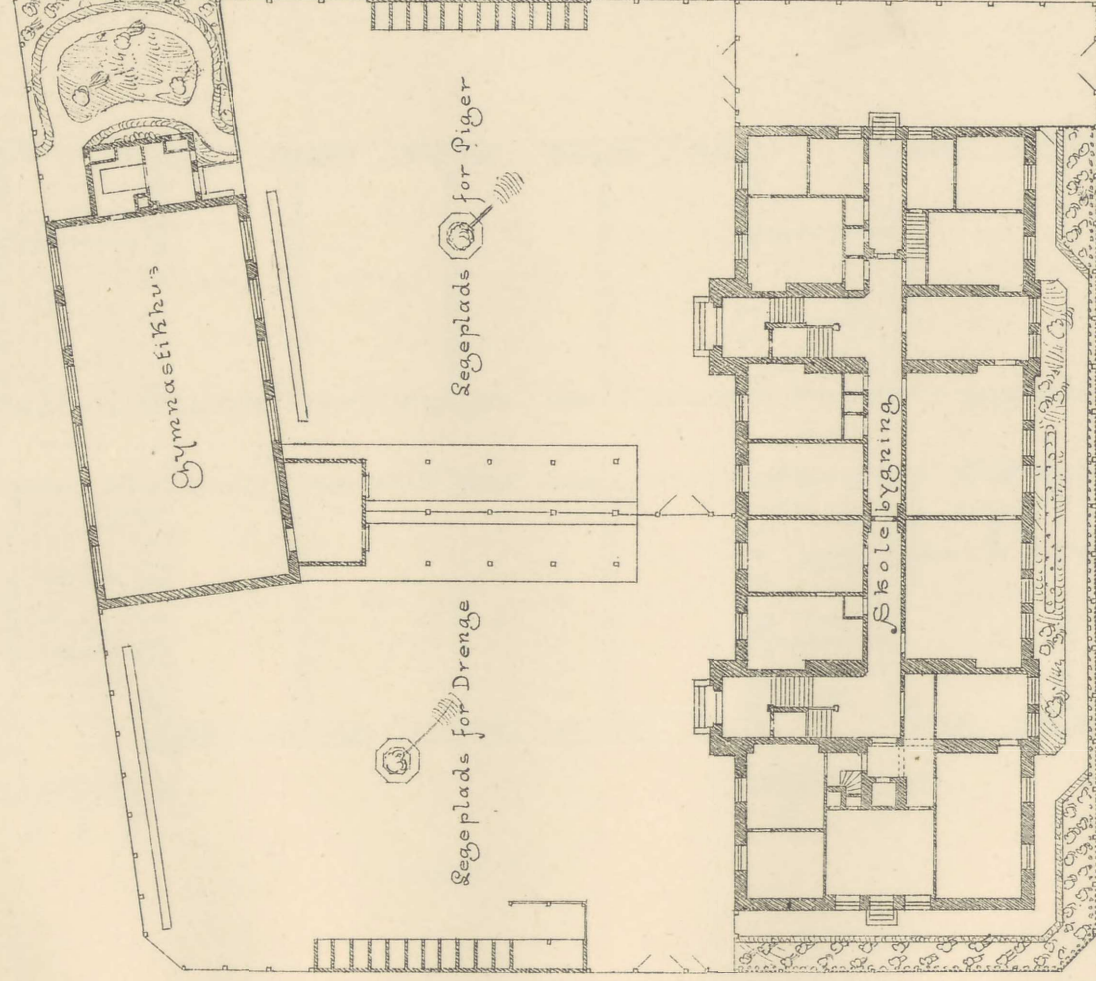
Situationsplan
