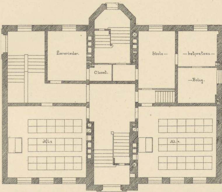
Plan of Stuen.
