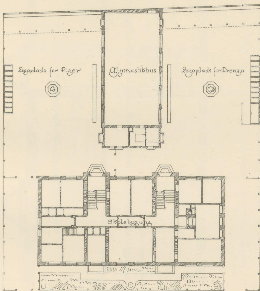
Situationsplan
