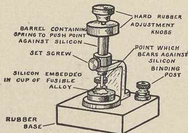
FIG. 71.—Silicon detector.
