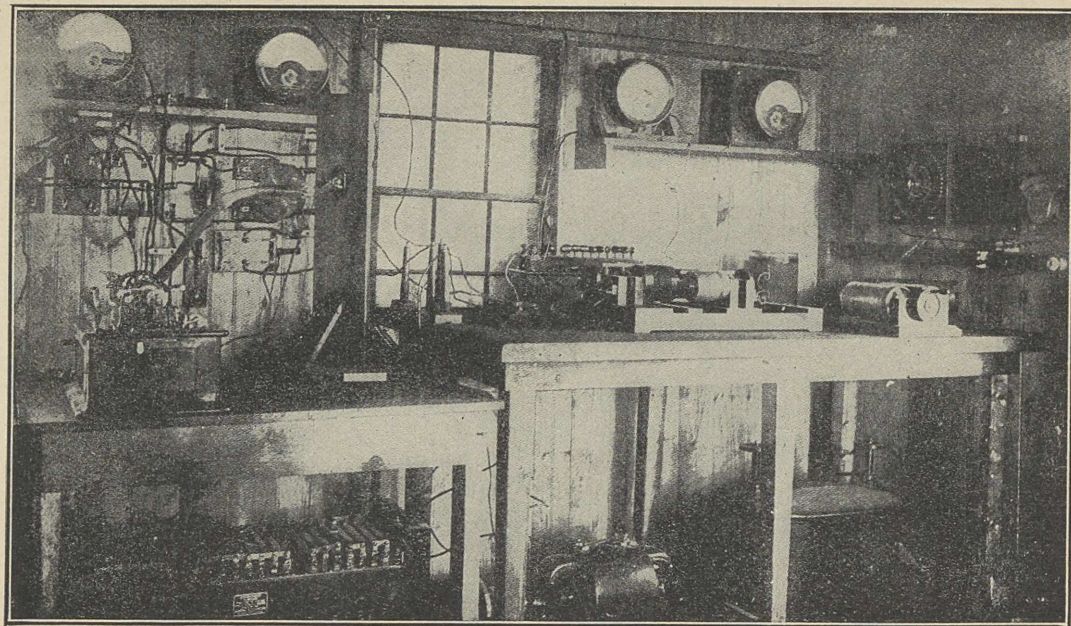
FIG. 142.—Fessenden wireless telephone transmitting phonograph music.
