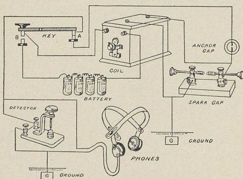
FIG. 118.—Breaking-in system.
