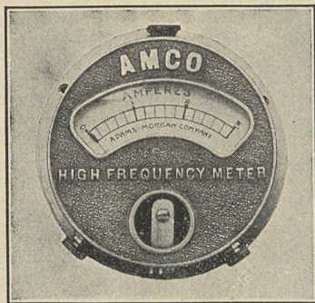
FIG. 88.—Hot-wire ammeter.
