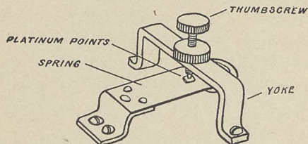
FIG. 37.—Interrupter for induction coil.
