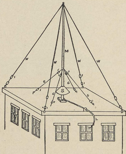
FIG. 21.—Umbrella aerial.
