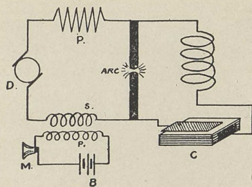
FIG. 145.—Arrangement of the speaking arc.
