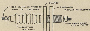
FIG. 26.—Leading-in insulator.
