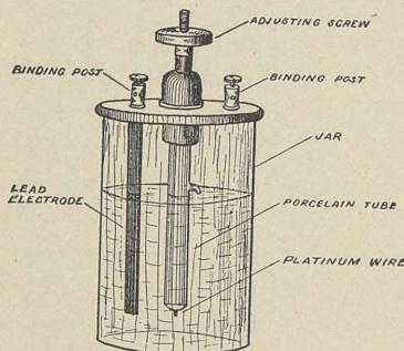
FIG. 38.—Electrolytic interrupter.
