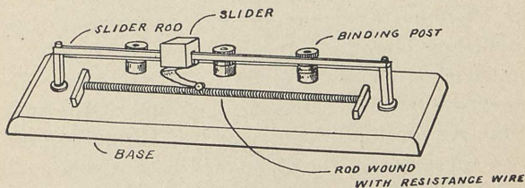
FIG. 74.—Potentiometer.
