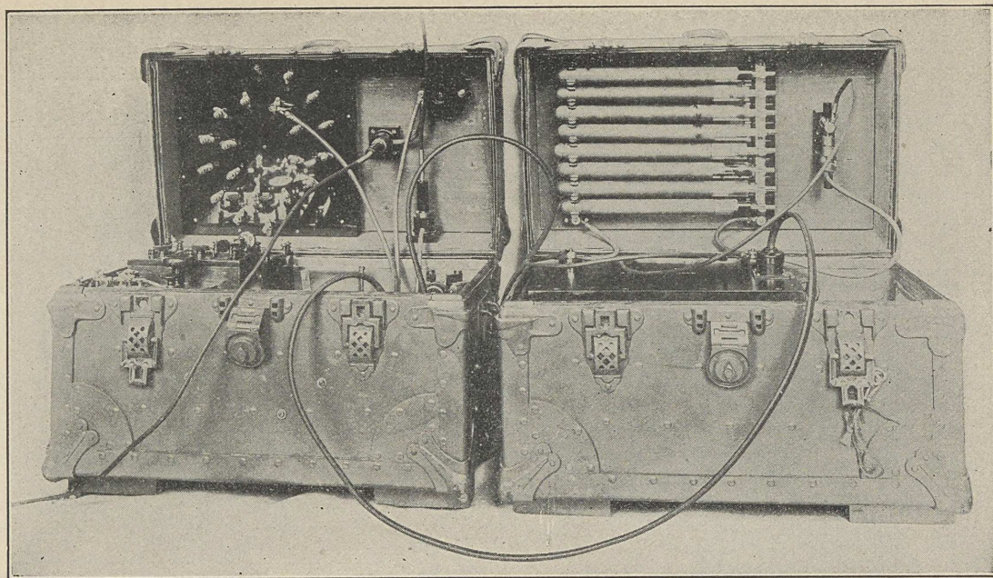
FIG. 62.—Portable pack set. The receiving outfit is contained in the left hand case; also the key and interrupter. The tubular condenser, spark gap, and induction coil may be seen in the right hand case.
