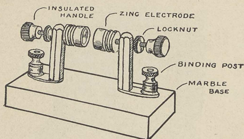
FIG. 50.—Spark gap.
