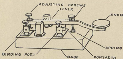
FIG. 57.—Wireless key.
