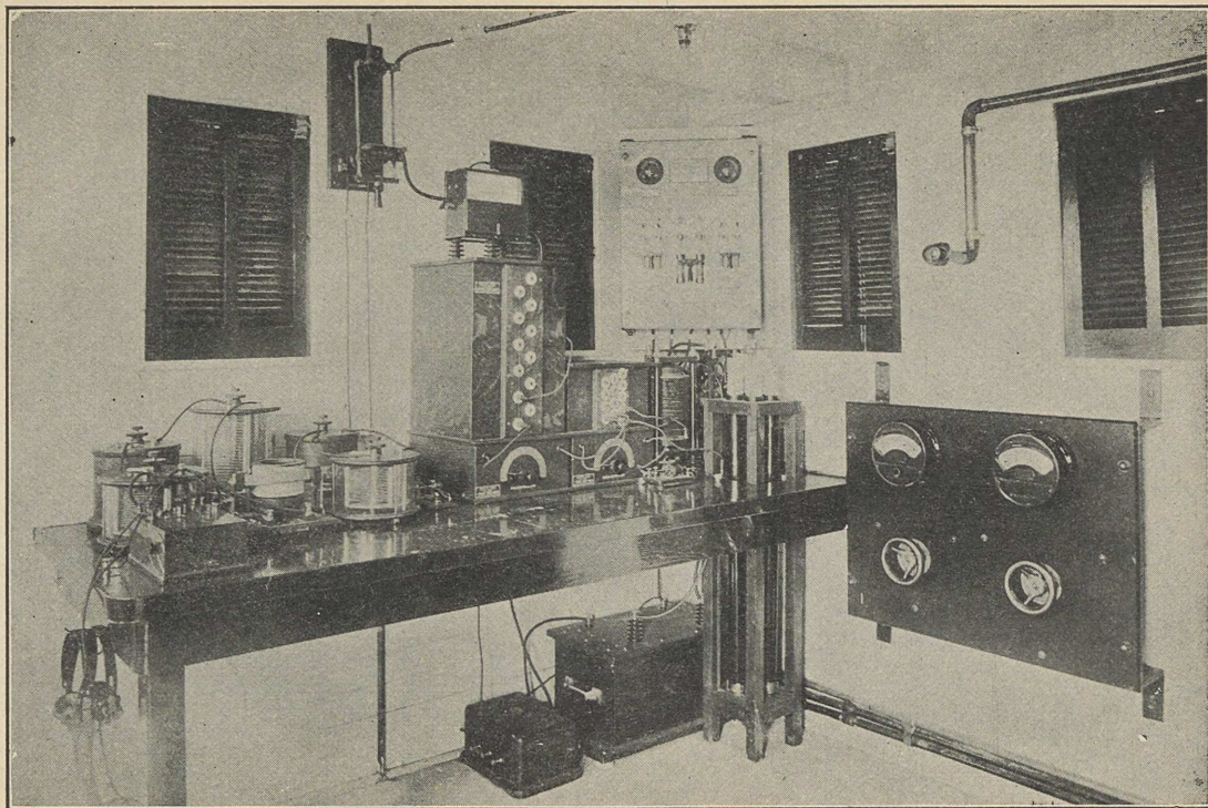
FIG. 104.—Wireless room aboard the U. S. transport "Buford."
