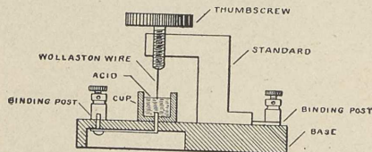
FIG. 72.—Electrolytic detector.
