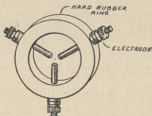
FIG. 56.—Anchor gap.
