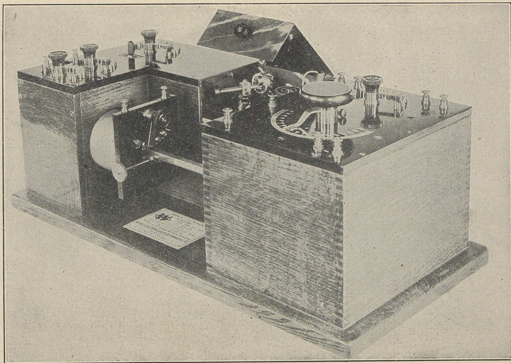
FIG. 63.—Complete receiving set, consisting of two “Perikon” detectors, potentiometer, loose coupler, variable condenser, etc.
