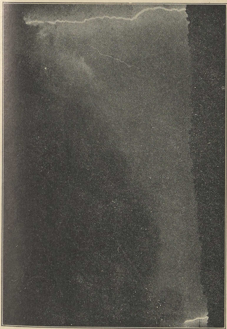
FIG. 14.—Photo of double lightning discharge passing to earth near the First Orange Mountain, Montclair, N. J.
