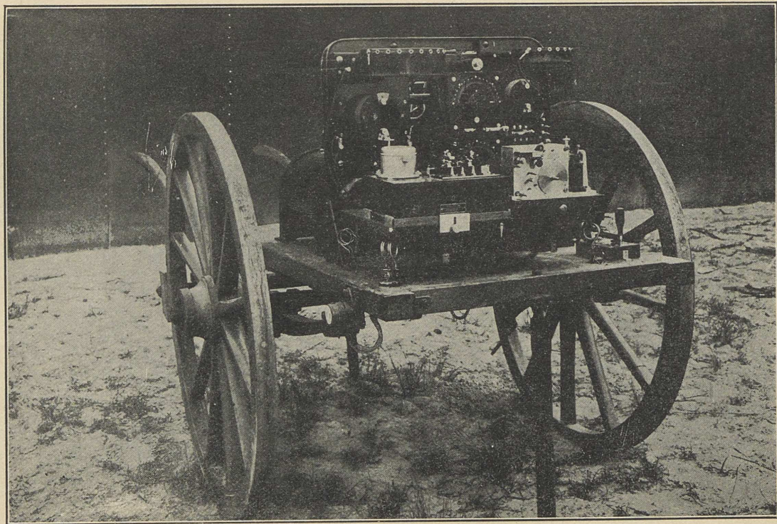
FIG. 102.—Telefunken wireless cart for military service, showing receiving apparatus.
