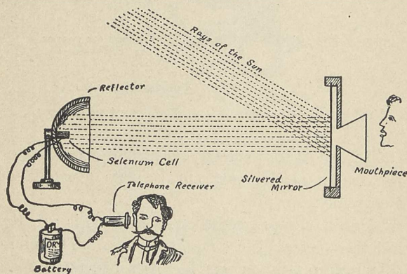
FIG. 133.—The photophone.
