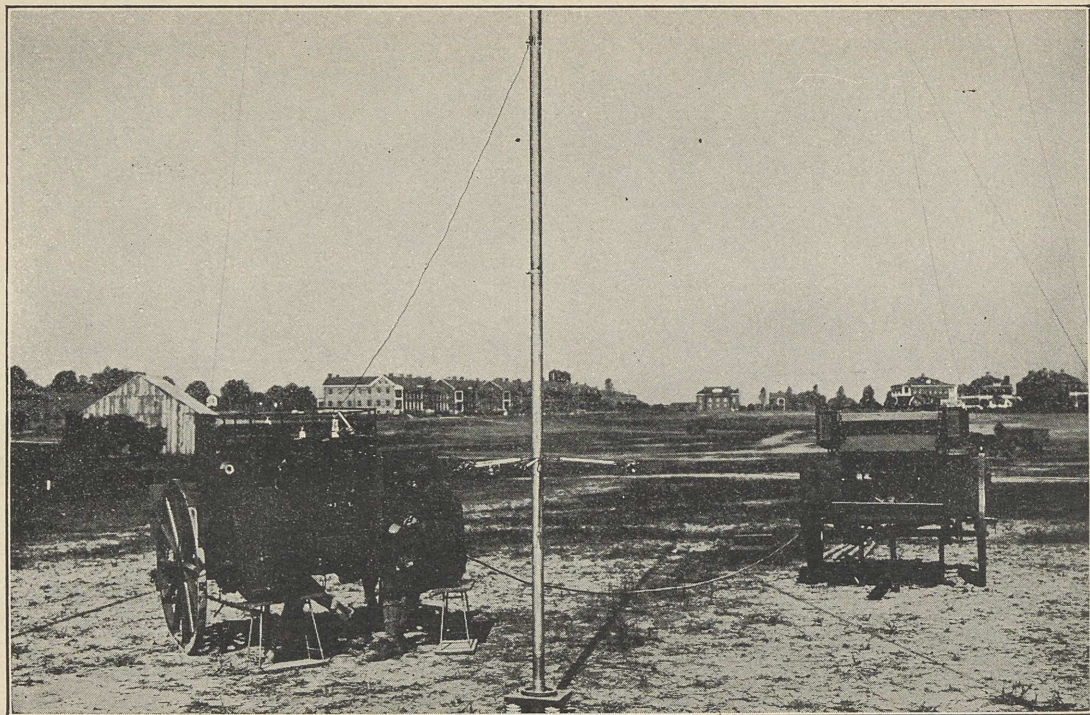
FIG. 103.—Telefunken wireless wagon set in operation at Fort Leavenworth, Kansas. The aerial is of the umbrella type supported by a steel pole resting on a porcelain base.
