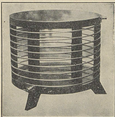
FIG. 49.—Close coupled helix.
