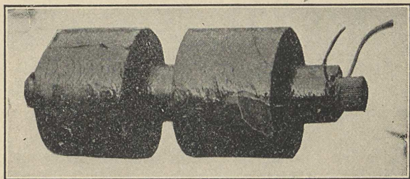
FIG. 36.—Induction coil, primary and secondary.
