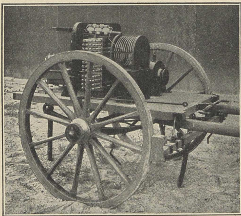
FIG. 101.—Telefunken wireless cart, showing transmitter.
