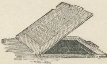
Fig. 5.—Book-form Double Dark Slide.
