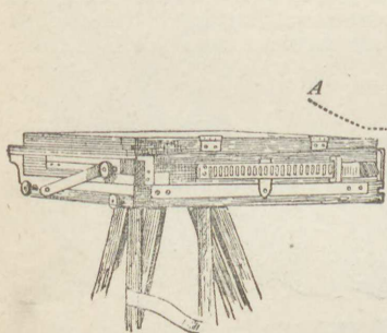
Fig. 1.—Closed Camera attached to Tripod.
