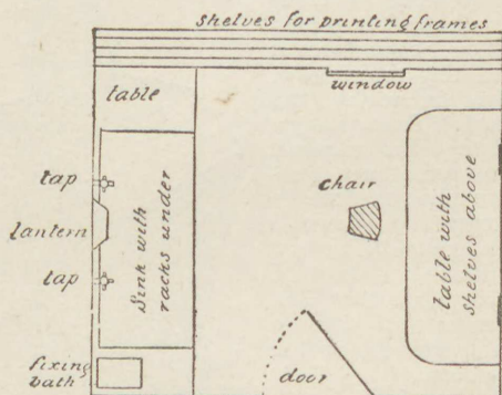
Plan of General Workroom.
