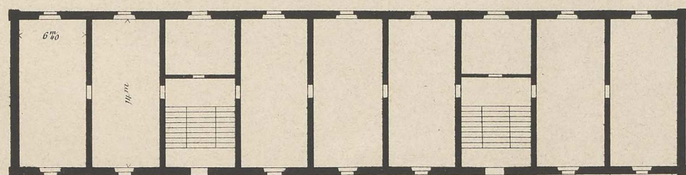
Fig 3 a 1:500.
