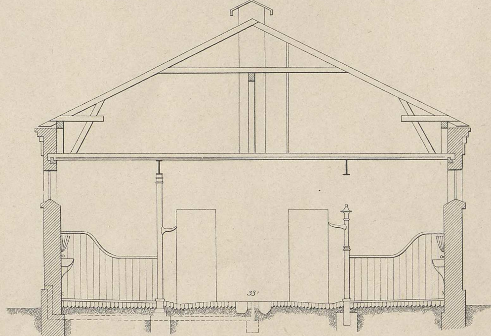
Fig 11 1:100.
