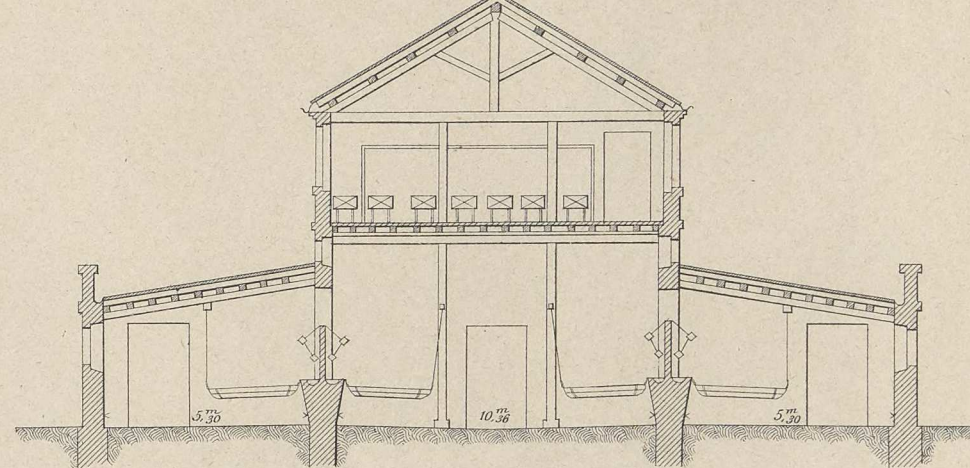
Fig 10 1:500.
