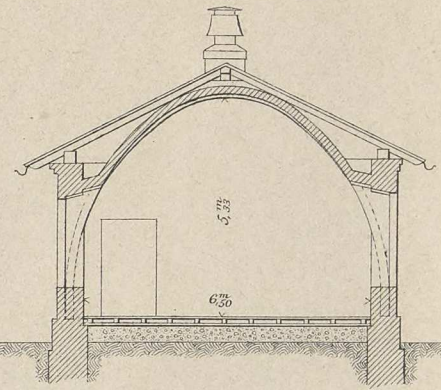
Fig 10 1:500.
